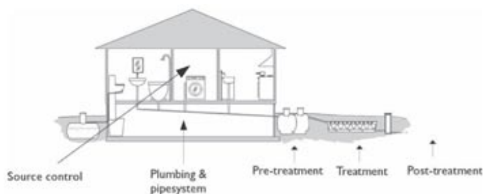
Technical components of a greywater management system
